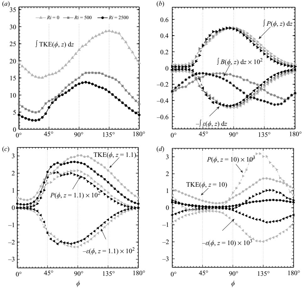
FIGURE 13. (a) Integrated (over z ) TKE normalized by u_{\tau, max}^2 \delta_s as function of phase. (b) Integrated production, integrated dissipation and integrated buoyancy flux over a half tidal cycle. Both are non-dimensionalized by u_{\tau, max}^2 U_0 . Light grey, dark grey and black are used for Ri = 0, 500 and 2500 , respectively. (c) TKE (normalized by u_{\tau, max}^2 ), production and dissipation as a function of phase at z = 1.1\delta_s for Ri = 0 (light grey) and Ri = 2500 (black). Both P and \epsilon are made non-dimensional by u_{\tau, max}^4 / \nu . (d) Same as in (c) for z = 10\delta_s .
