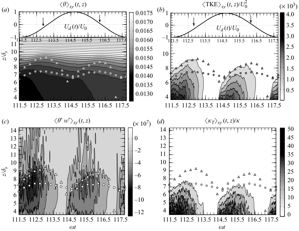
FIGURE 6. Contours, as a function of z and t , in case 3 with Ri = 2500 that illustrate the behaviour of the thermal statistics over a half-cycle. The symbol \circ denotes the location of \partial \langle \theta \rangle_{xy}(z, t) / \partial z = 0.1 while the symbol \triangle locates Ri_g(z, t) = 0.25 . The two upper insets show the background velocity with two downward arrows that show the locations of the local maxima of the mixed layer height h_m . (a) Plane-averaged temperature; (b) Plane-averaged TKE normalized by U_0^2 ; (c) Plane-averaged vertical heat flux, \langle \theta' w' \rangle_{xy}(z, t) normalized by U_0^2 d\theta/dz|_{\infty}/\omega ; (d) Eddy diffusivity, \kappa_T(z, t) normalized by molecular diffusivity \kappa .
