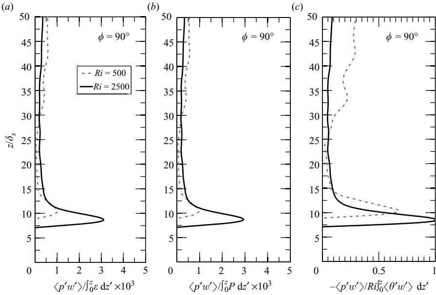
FIGURE 24. Vertical energy flux normalized by (a) the integrated turbulent dissipation, (b) the integrated production and (c) the integrated buoyancy flux at \phi = 90^\circ for Ri = 500 and 2500 .
